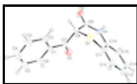
Fig. 1. View of the title compound with the atom numbering scheme. The thermal ellipsoids are drawn at the 30% probability level. H-atoms are shown by small circles of arbitrary radii.
