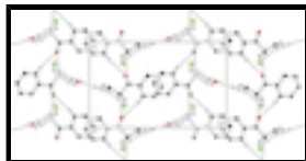
Fig. 2. The partial packing ( PLATON ; Spek, 2009) which shows that molecules form dimers which are interlinked in the form of polymeric sheets. The H-atoms not involved in H-bondings are omitted for clarity.
